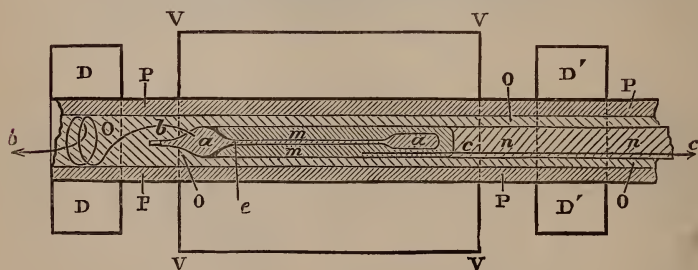
Fig. 2.—Diagram of Tube in place.
