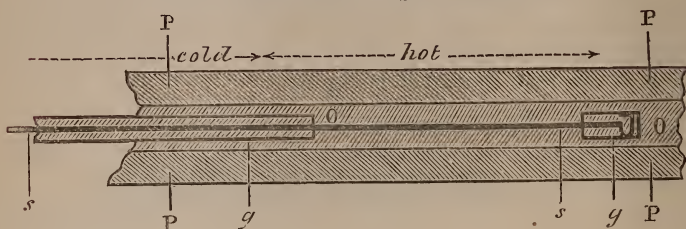
Fig. 4.—Arrangement for measuring the Pressure Increments of the Electric Resistance of Liquid Insulators.
