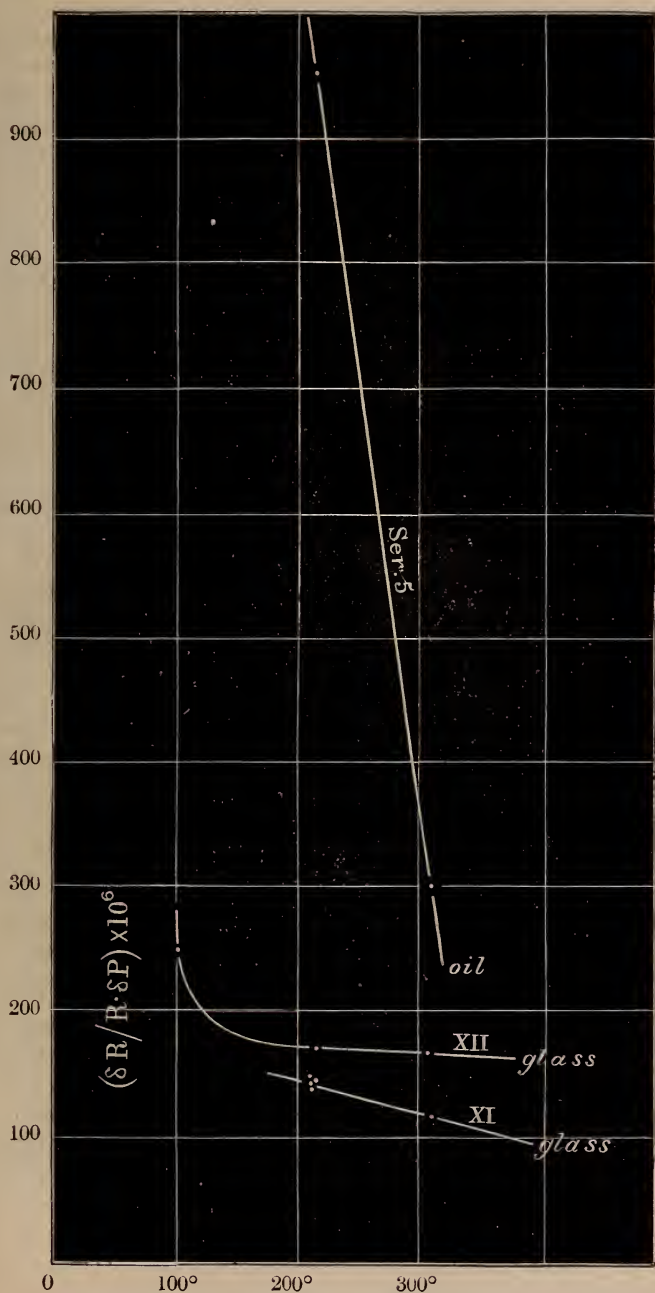
Fig. 5.--Charts showing the Relation of Pressure-Coefficient and Temperature for Glass and Hydrocarbon Oil ("mineral sperm").
