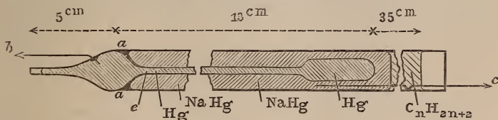
Fig. 1.—Tube for measuring the Pressure-increments of the Electric Resistance of Glass.
