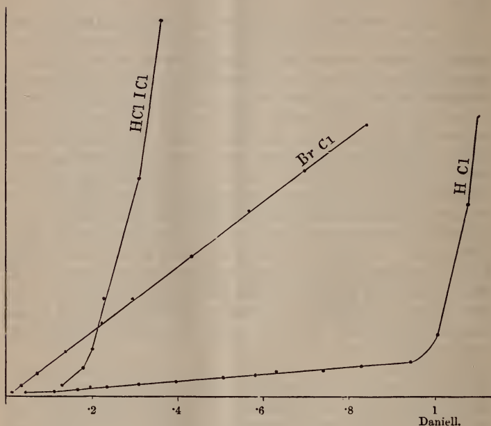
Fig. 3.—Electrolysis of Aqueous Solutions of Hydrogen-Iodine Chloride, Bromine Chloride, and Hydrochloric Acid. Abscissæ correspond to electromotive force in parts of a Daniell; ordinates to current as measured by deflexions of a reflecting-galvanometer (the larger values are about 5 per cent. too large on this instrument).
