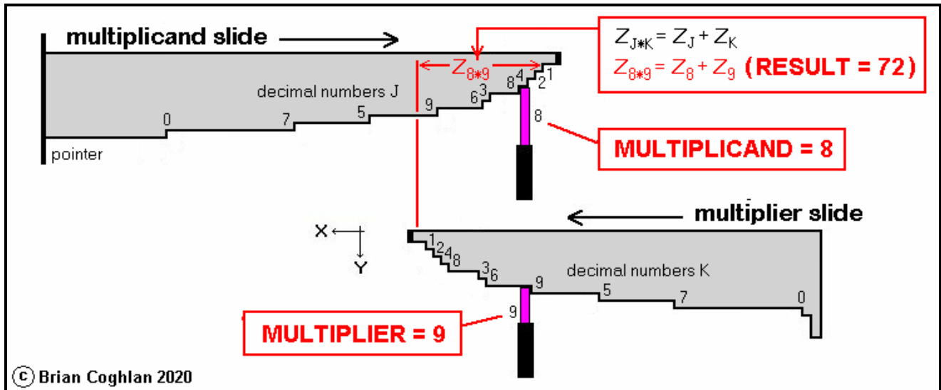
FIG. 4—Multiplication using Ludgate’s logarithmic slides for calculation of 8*9 = 72 (Image courtesy of The John Gabriel Byrne Computer Science Collection).
