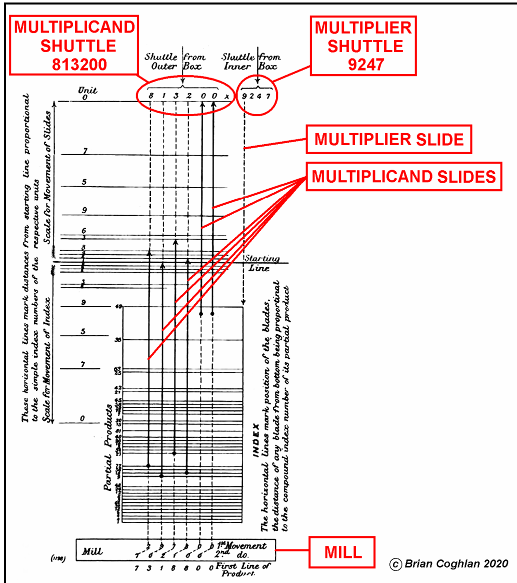
FIG. 3—Annotated version of the diagram from Engineering, 20 August 1909, pp.256-7 (Image courtesy of The John Gabriel Byrne Computer Science Collection).
