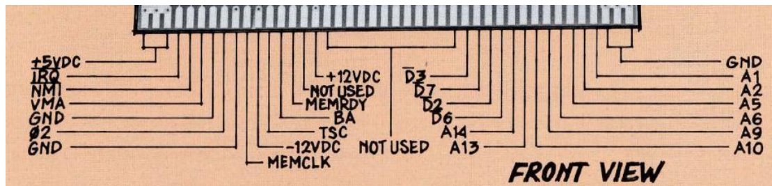
Figure 12: Motorola EXORbus front pinout
