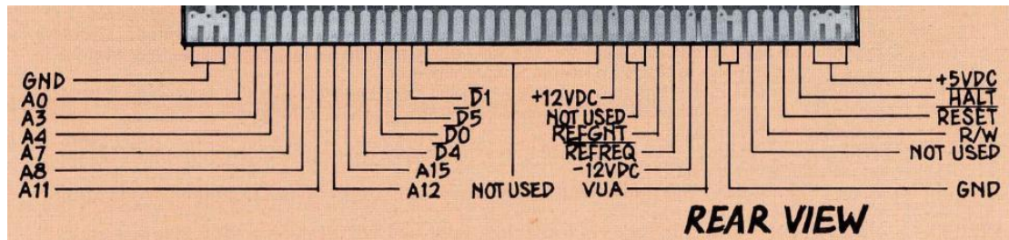
Figure 13: Motorola EXORbus rear pinout
