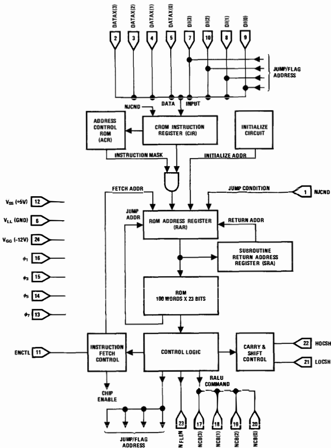
FIGURE 1. CROM Block Diagram
