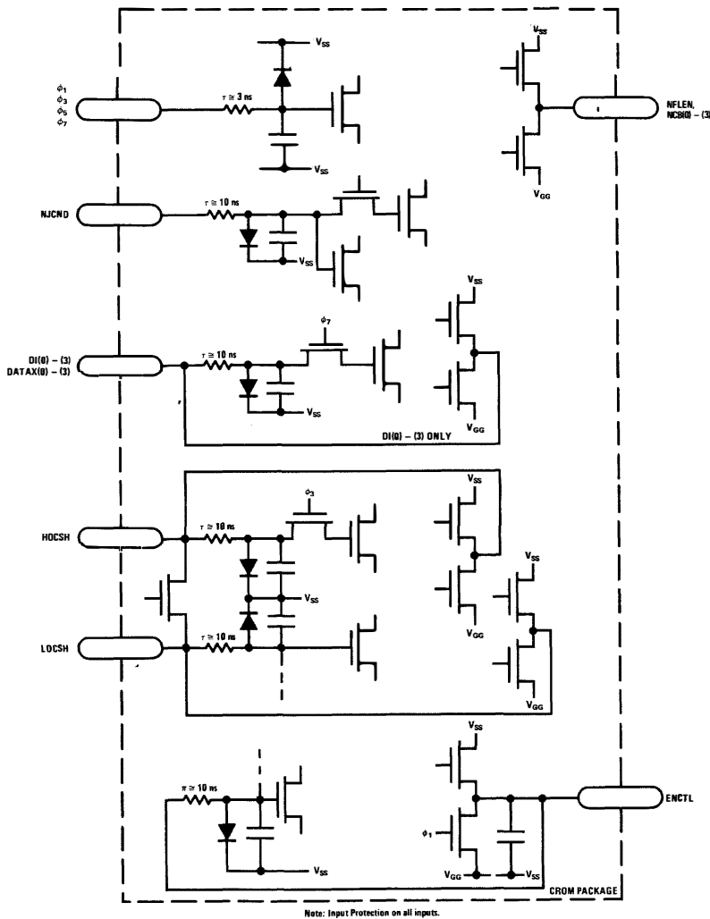
FIGURE 3. CROM Driver and Receiver Buffer
