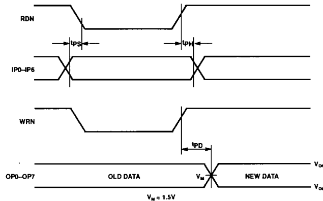
Figure 3. Port Timing
