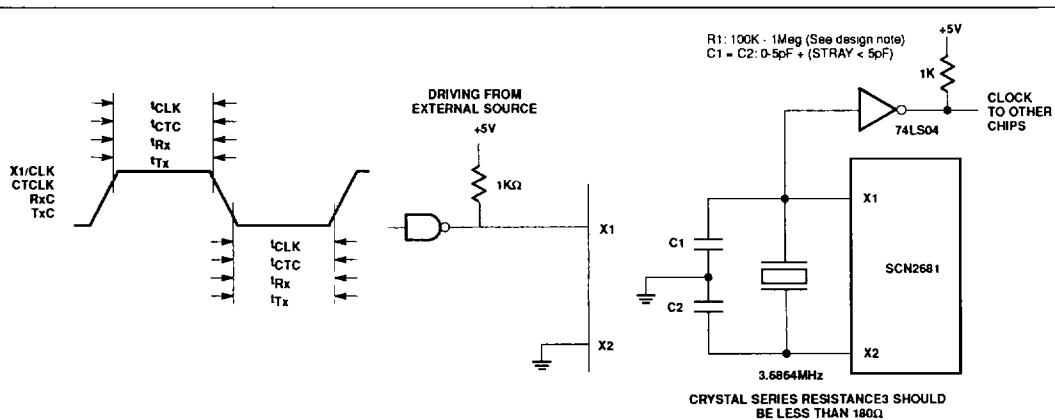
Figure 5. Clock Timing
