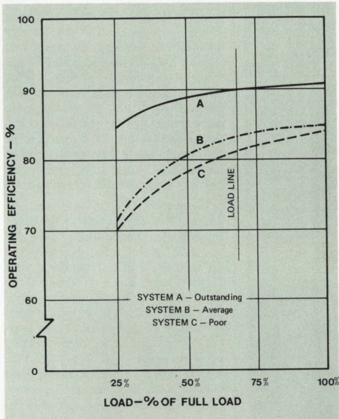
Fig. 1 - Efficiency deterioration curves for three systems from 25 percent to 100 percent of full load. Note rapid deterioration in efficiency of Systems B and C at fractional loads. System C is typical for the better motor-generator frequency converters.
