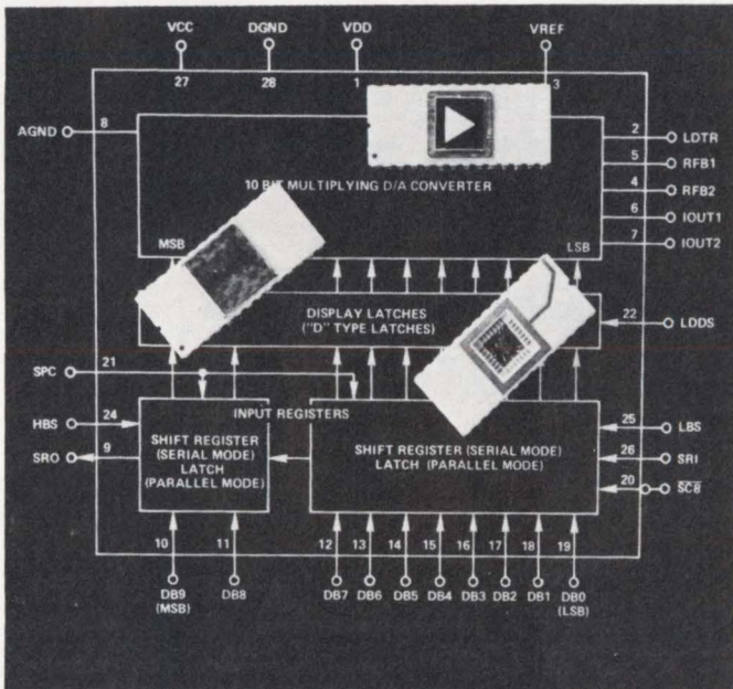
Analog Devices directly-interfaceable buffered D/A converter.
