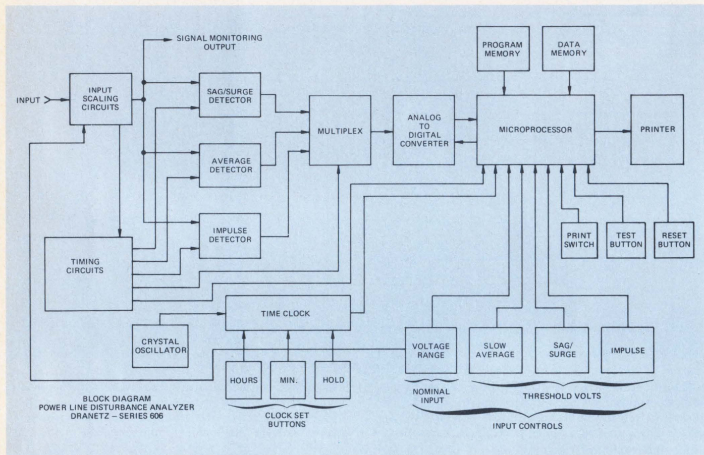
Fig. 3 - Analogic functional block diagram
