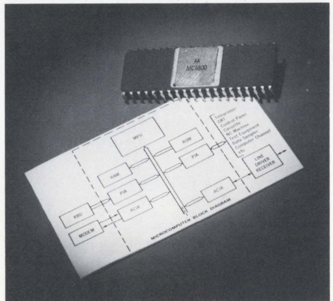
Motorola's MC6800 microprocessor and its functional block diagram.
