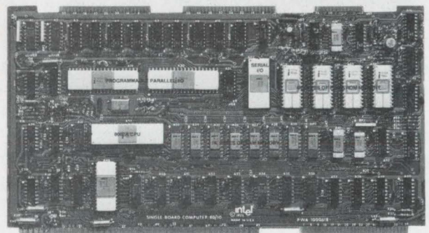
Intel's SBC-80/10 Single-Board Computer.
