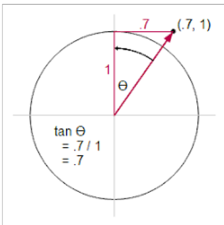
Arctan in the Sinclair Scientific works by measuring the rotation angle required to make the vector vertical.
