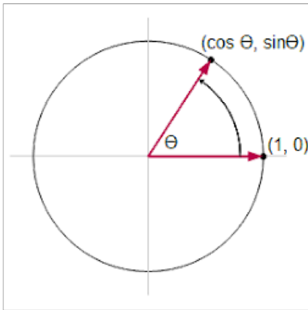
Vector rotation is used to compute sine and cosine in the Sinclair Scientific calculator.
