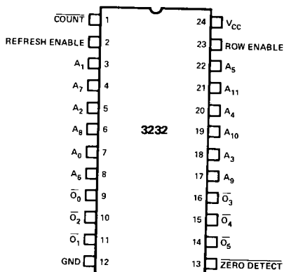
PIN CONFIGURATION
