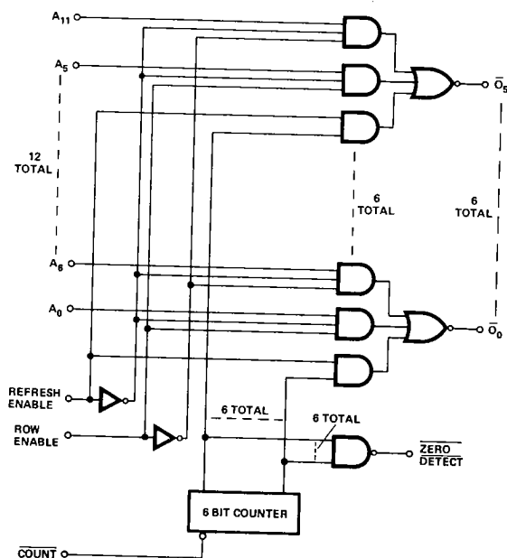
LOGIC DIAGRAM
