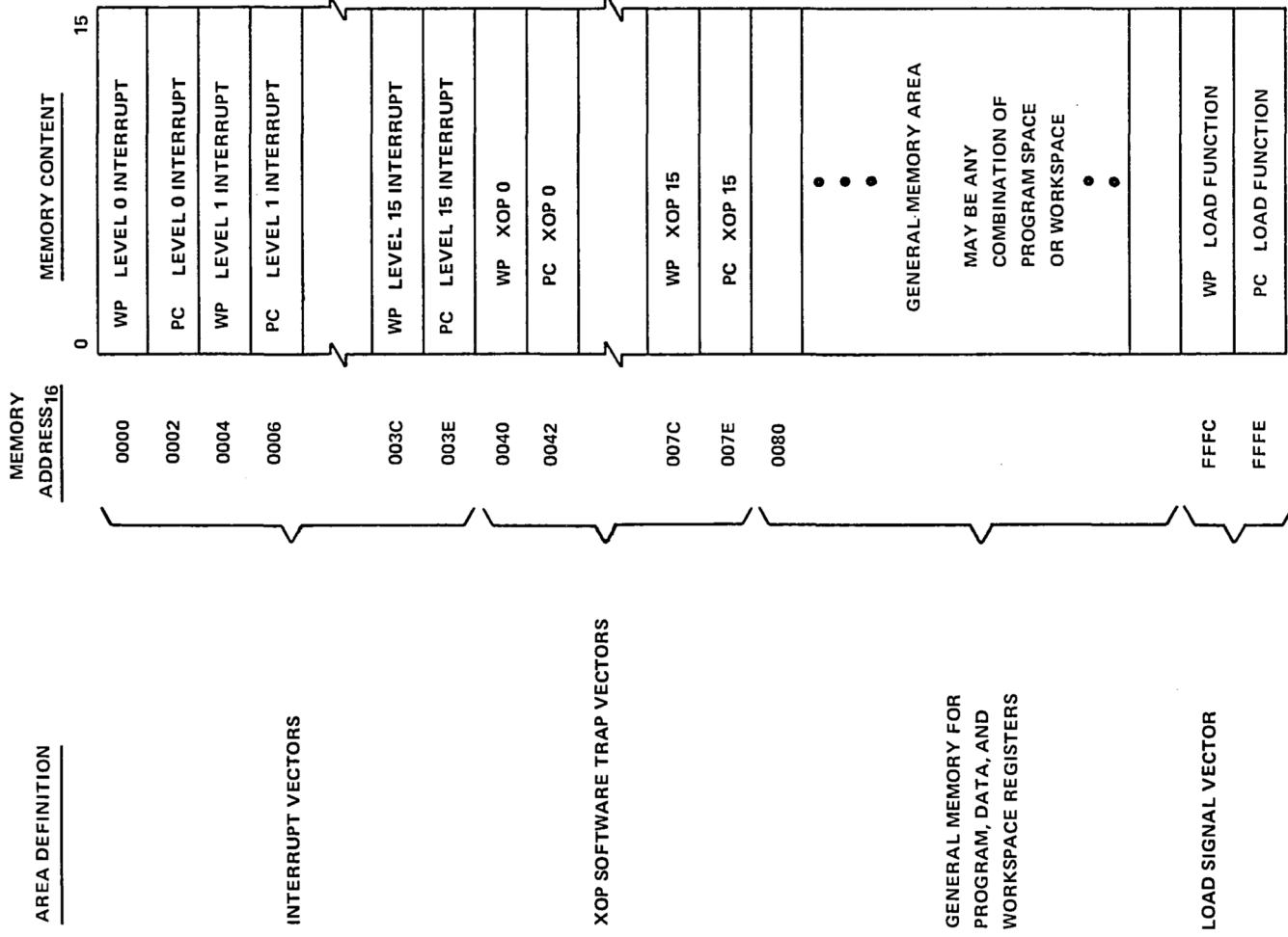
FIGURE 2 – MEMORY MAP
