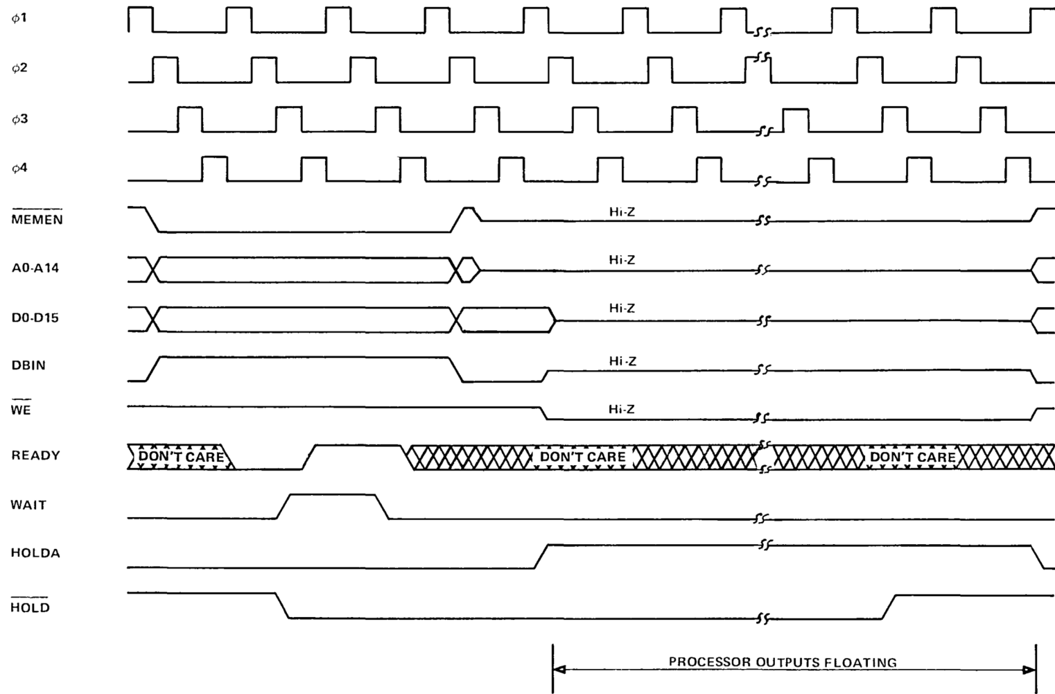
FIGURE 10 – TMS 9900 HOLD TIMING
