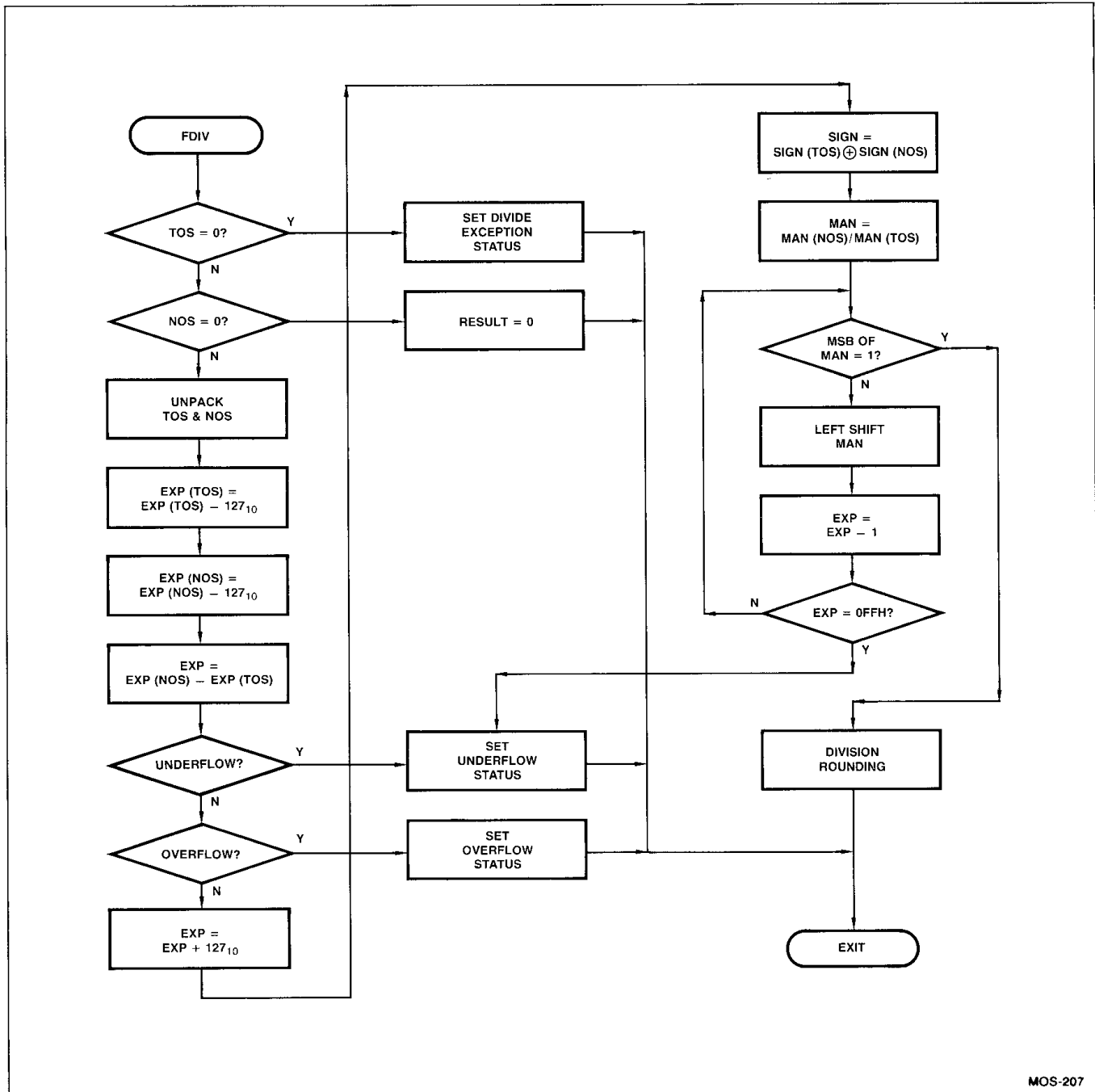
Figure 3.3. Floating Point Divide Flowchart
