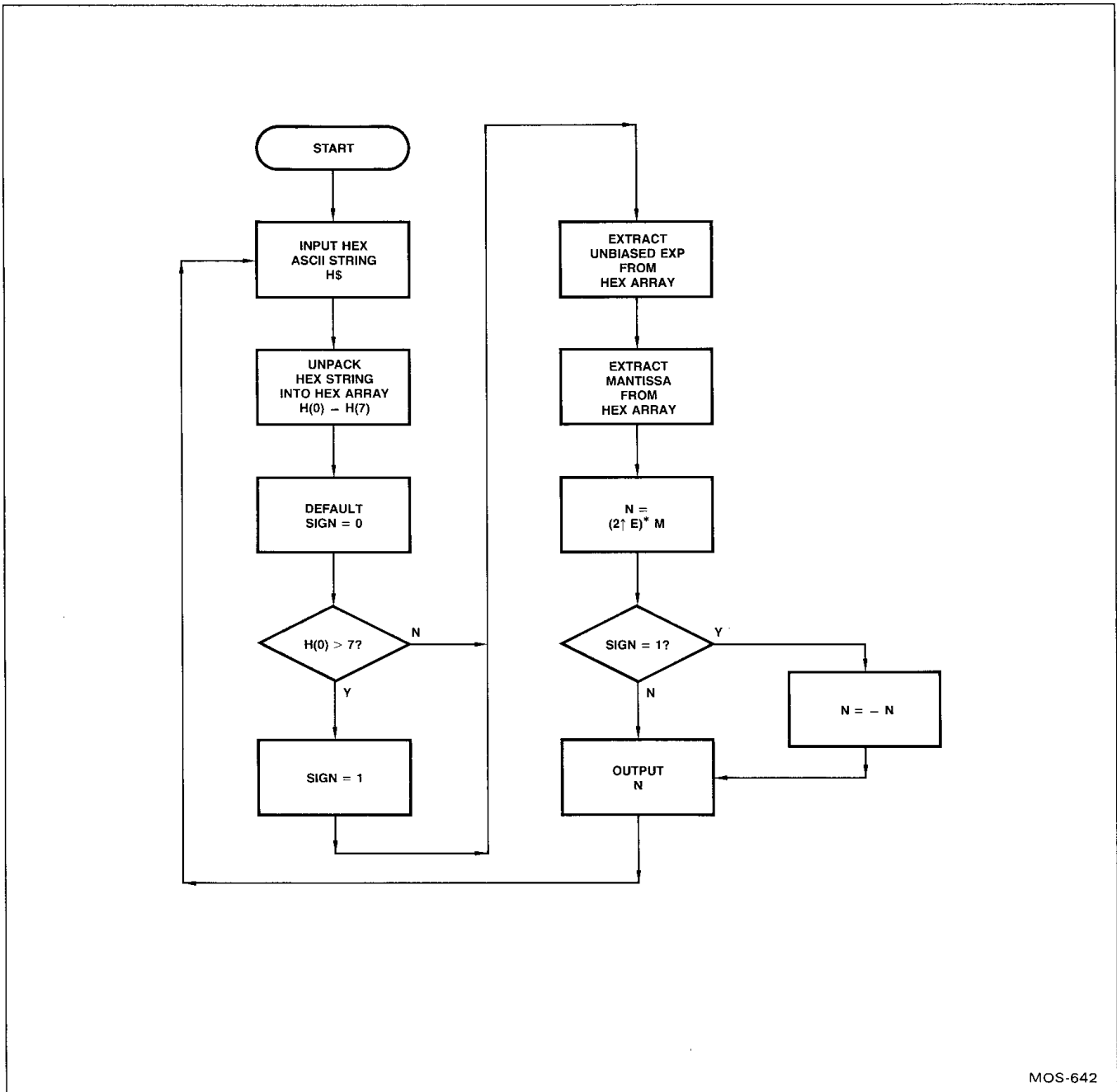
Figure 4.6. Binary to Decimal Floating Point Conversion Flowchart
