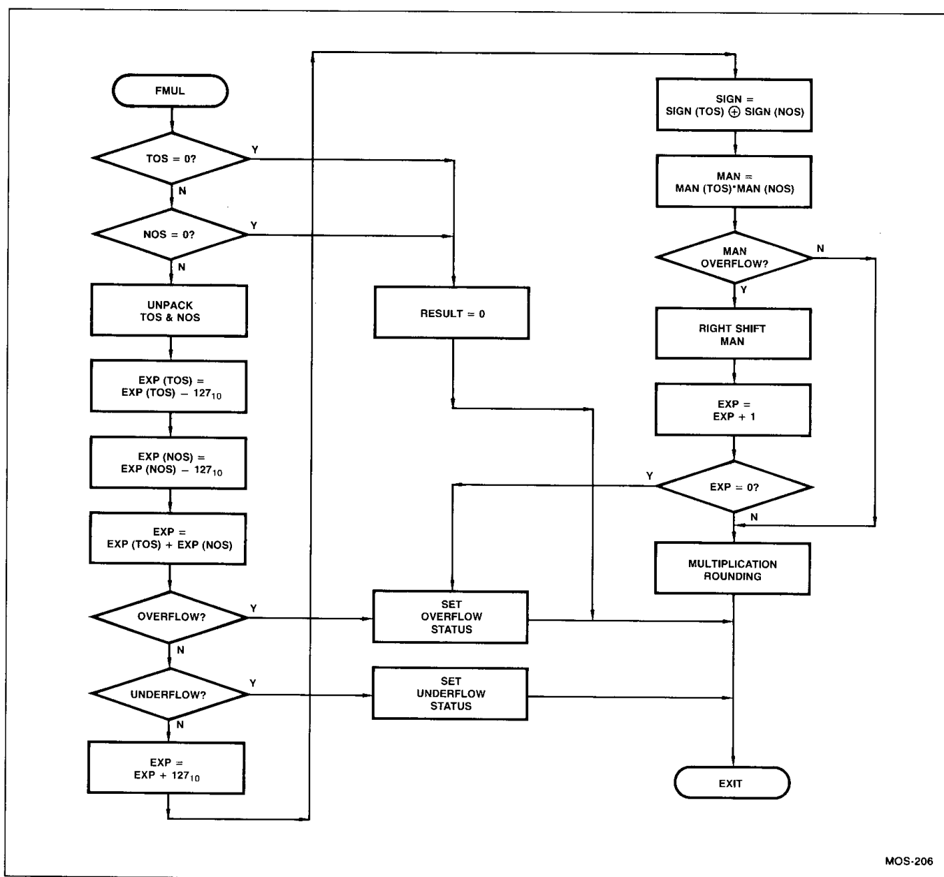
Figure 3.2. Floating Point Multiply Flowchart
