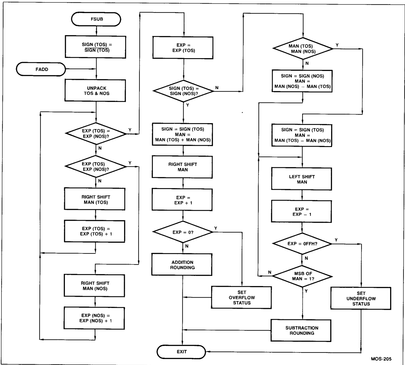
Figure 3.1. Floating Point Add/Subtract Flowchart
