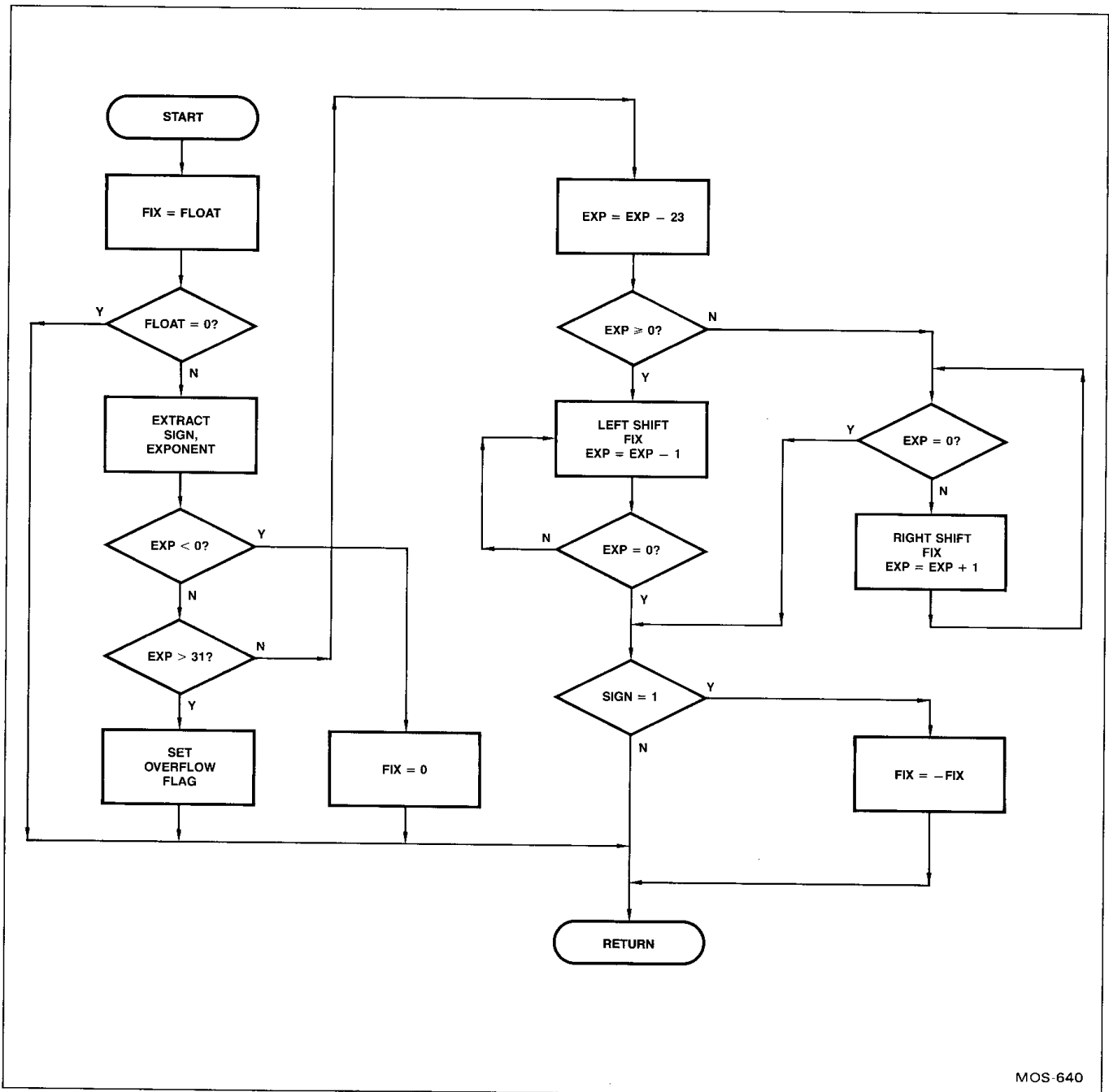
Figure 4.3. Fix to Float/Float to Fix Conversion Subroutines
