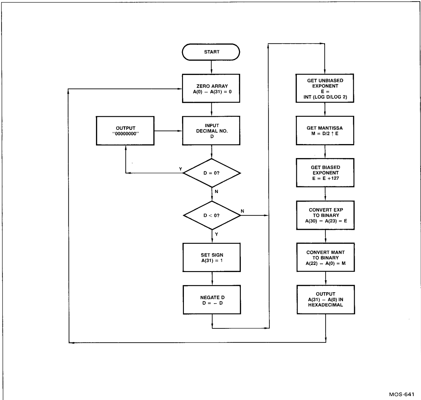
Figure 4.4. Decimal to Binary Floating Point Conversion Flowchart
