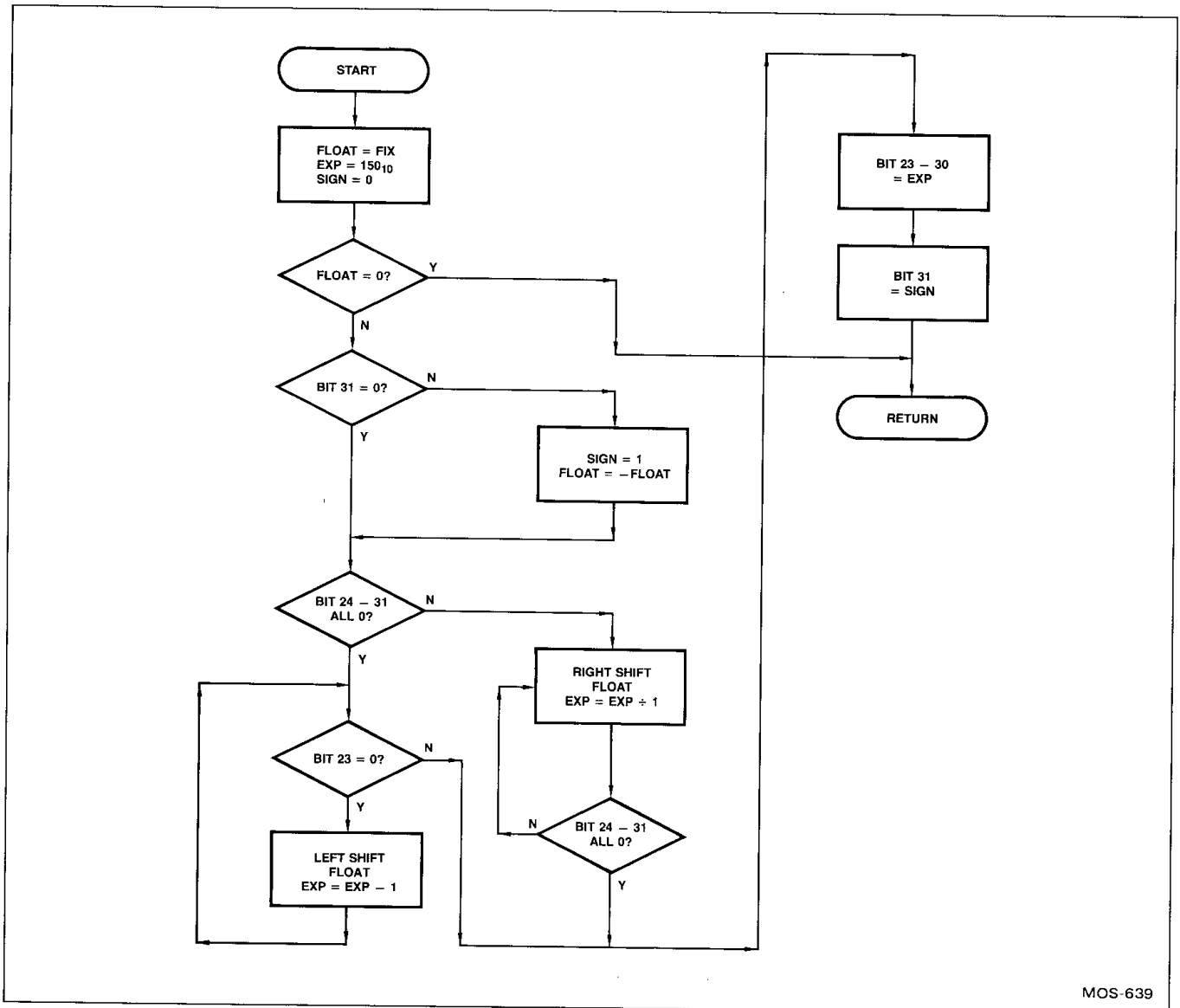
Figure 4.1. Fix to Float Conversion Flowchart
