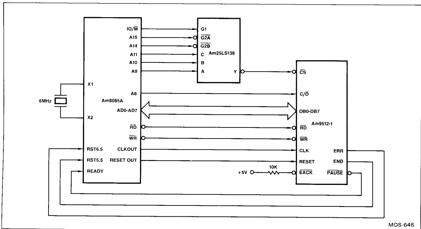
Figure 6.4. Am8085A to Am9512-1 Interface
