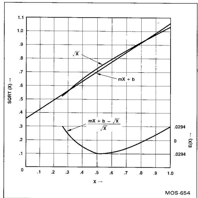
Figure 9.5. Square Root Computation
