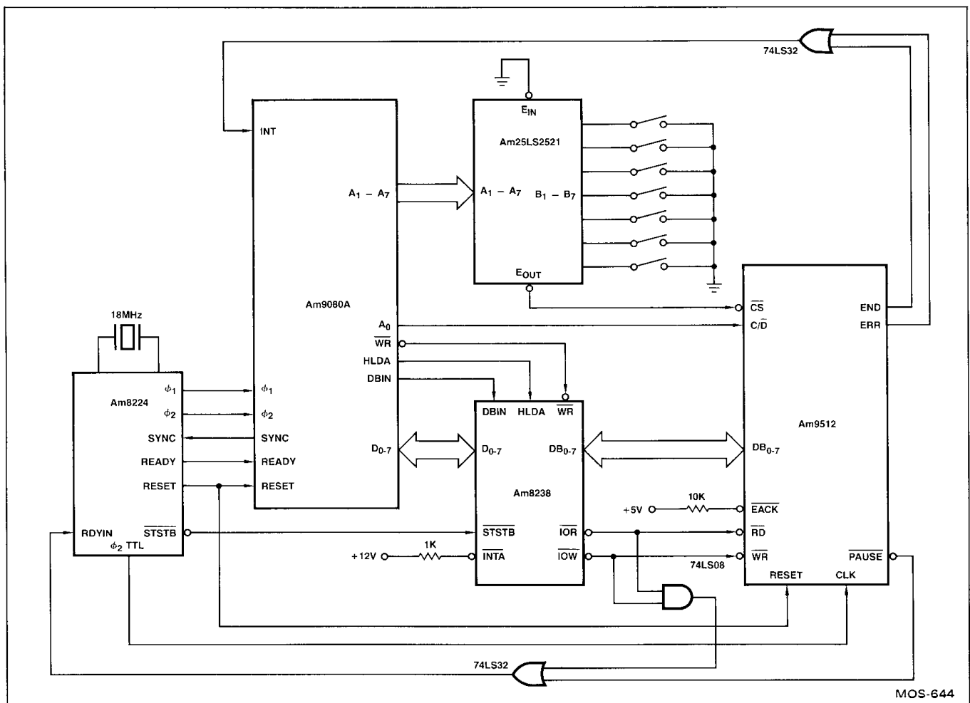
Figure 6.2. Am9080A to Am9512 Interface
