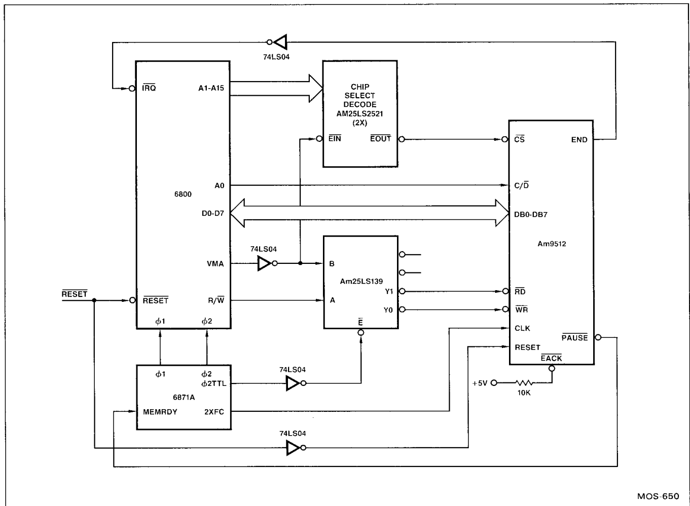
Figure 6.8. MC6800 to Am9512 Interface
