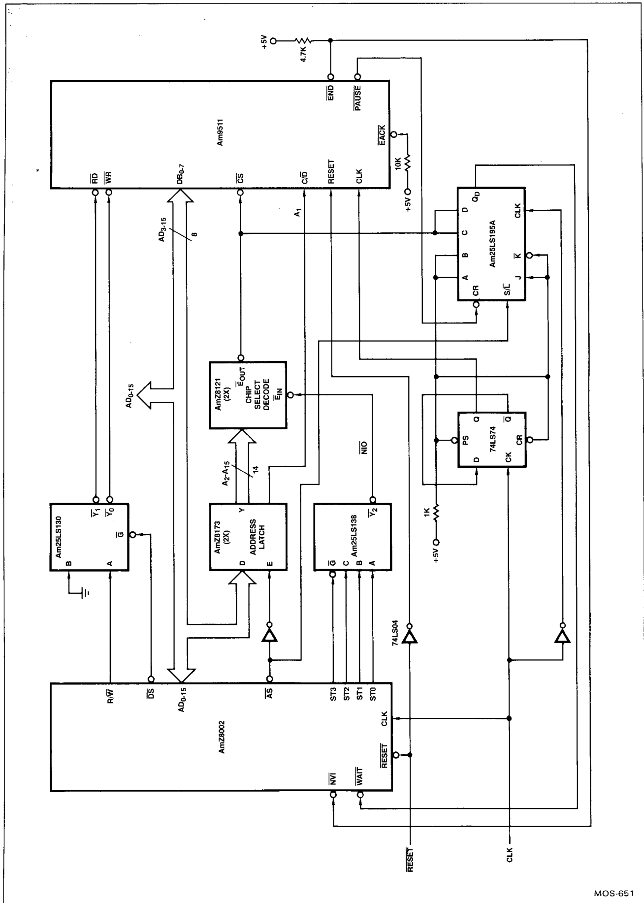
Figure 6.9. AmZ8002 to Am9511A Interface
