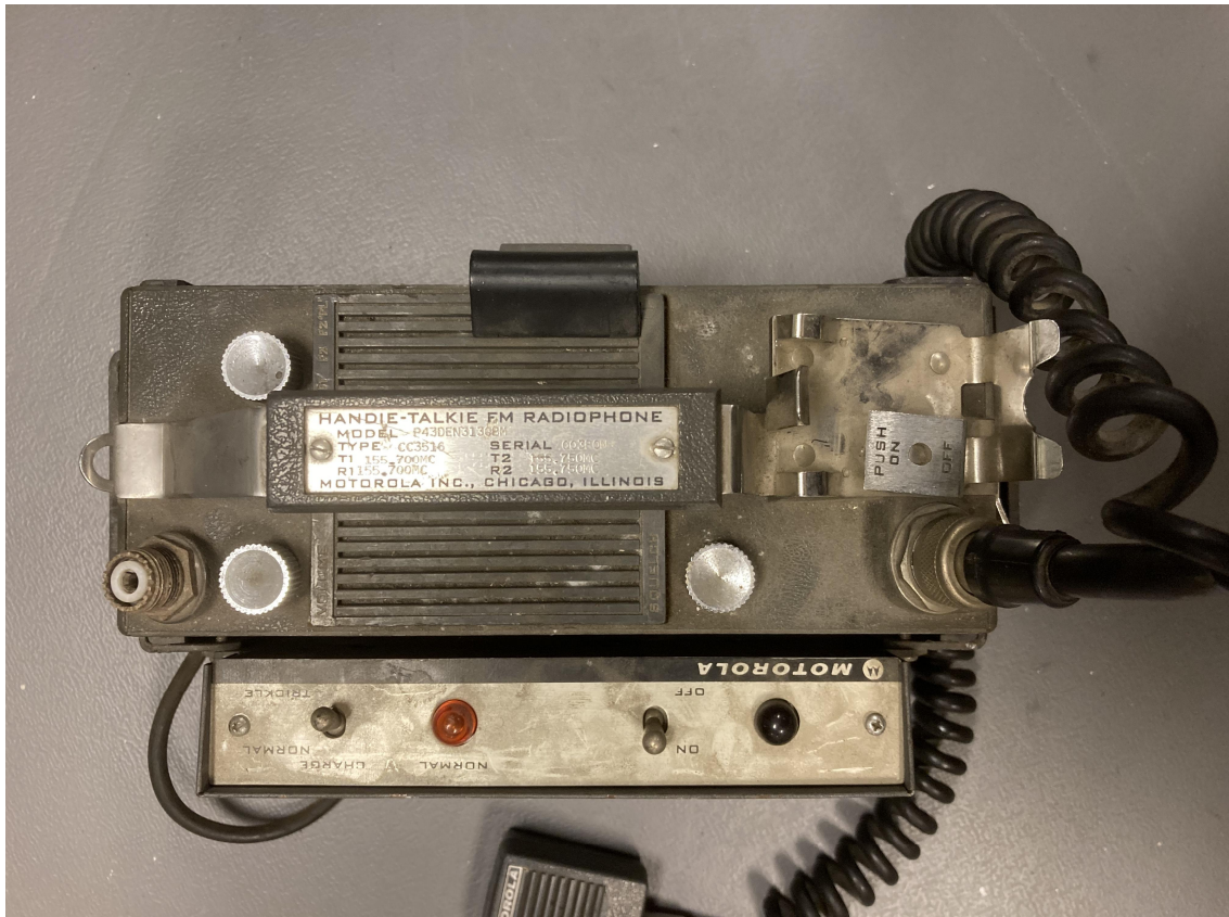
Figure 3: Motorola PT400 top view
