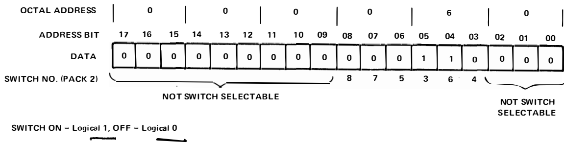
Figure 4-11 DL11-W Vector Address Selection
