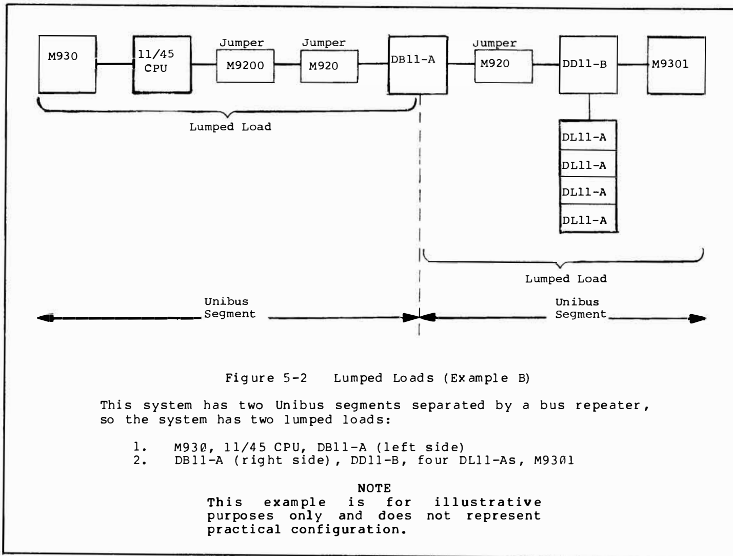
Figure 5-2. Lumped Loads (Example B)
