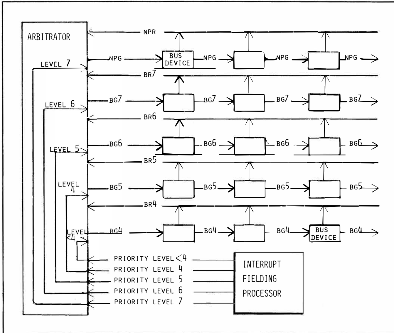
Figure 3-2. Priority Structures Block Diagram
