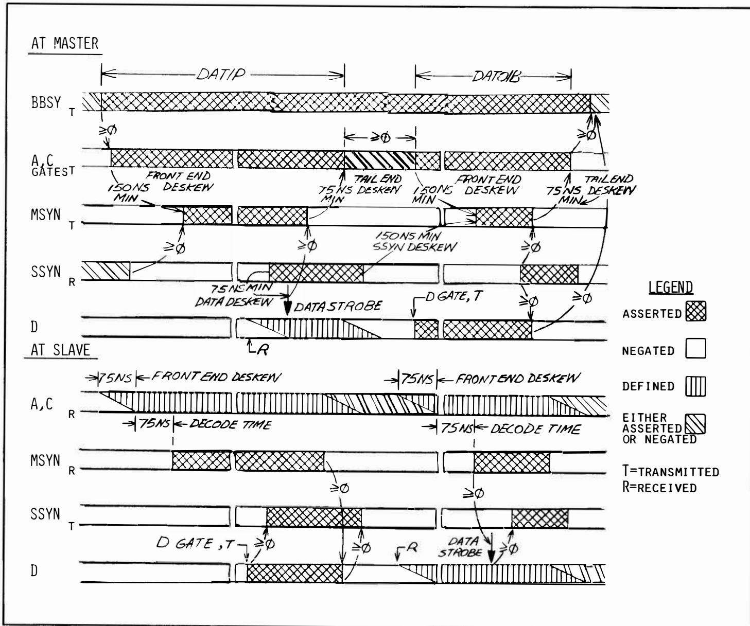
Figure 3-12. Typical DATIP-DATO/B Transaction (See Paragraph 3.1.4)
