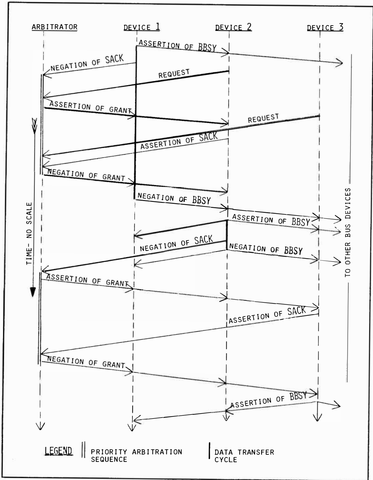
Figure 3-4. Typical Arbitration Sequence
