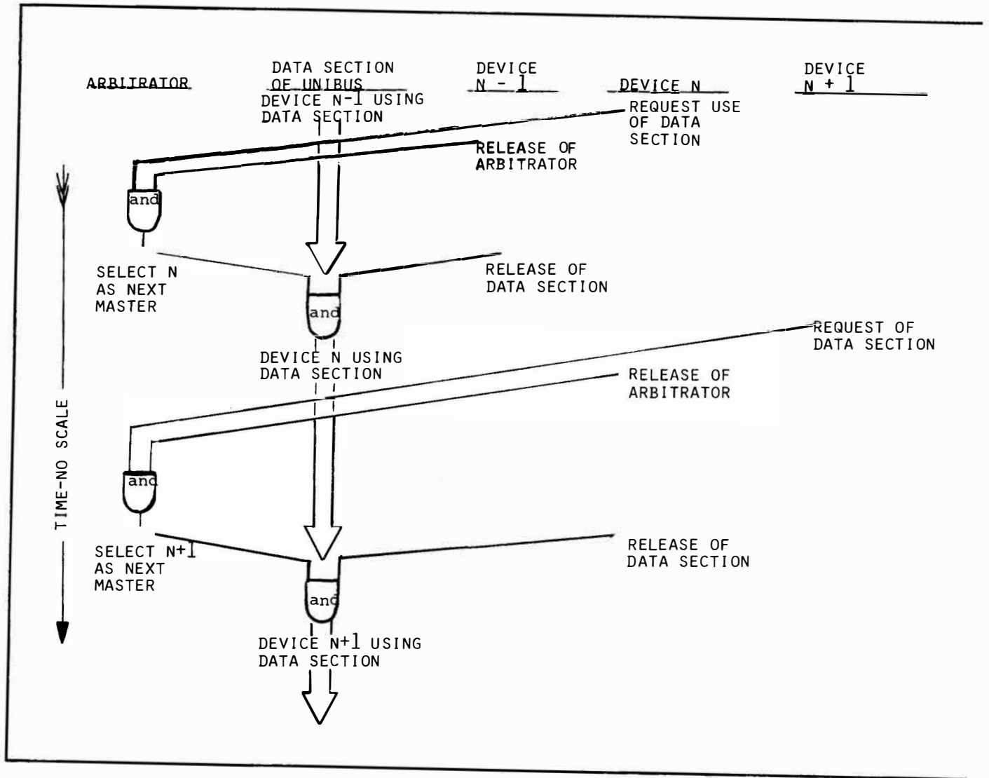
Figure 3-1. Unibus Block Diagram
