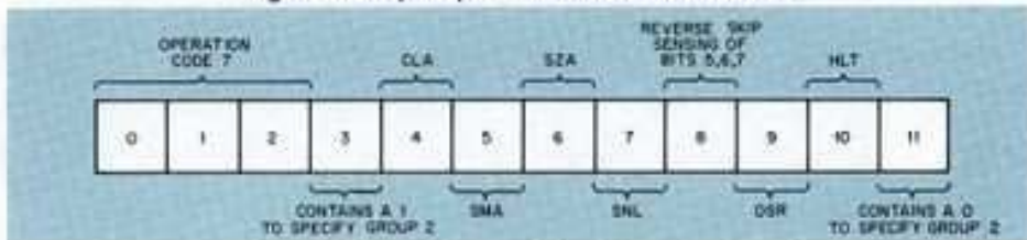
Figure 7 Group 2 Operate Microinstruction Format
