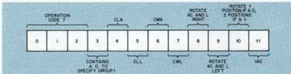
Figure 6 Group 1 Operate Microinstruction Format
