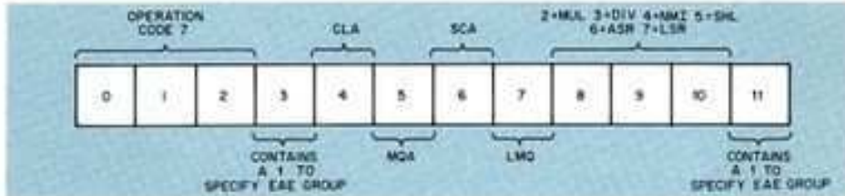
Figure 8 EAE Microinstruction Format
