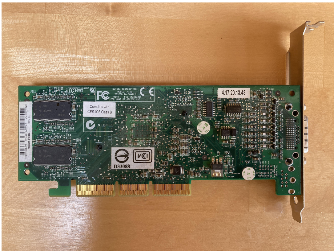
Figure 4: nVidia P150 GPU Card, bottom view TCD-SCSS-T.20121208.134.02
