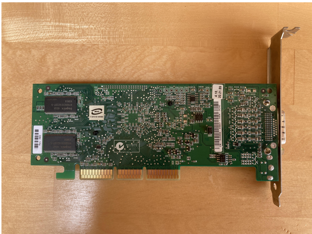
Figure 2: nVidia P118 GPU Card, bottom view TCD-SCSS-T.20121208.134.01
