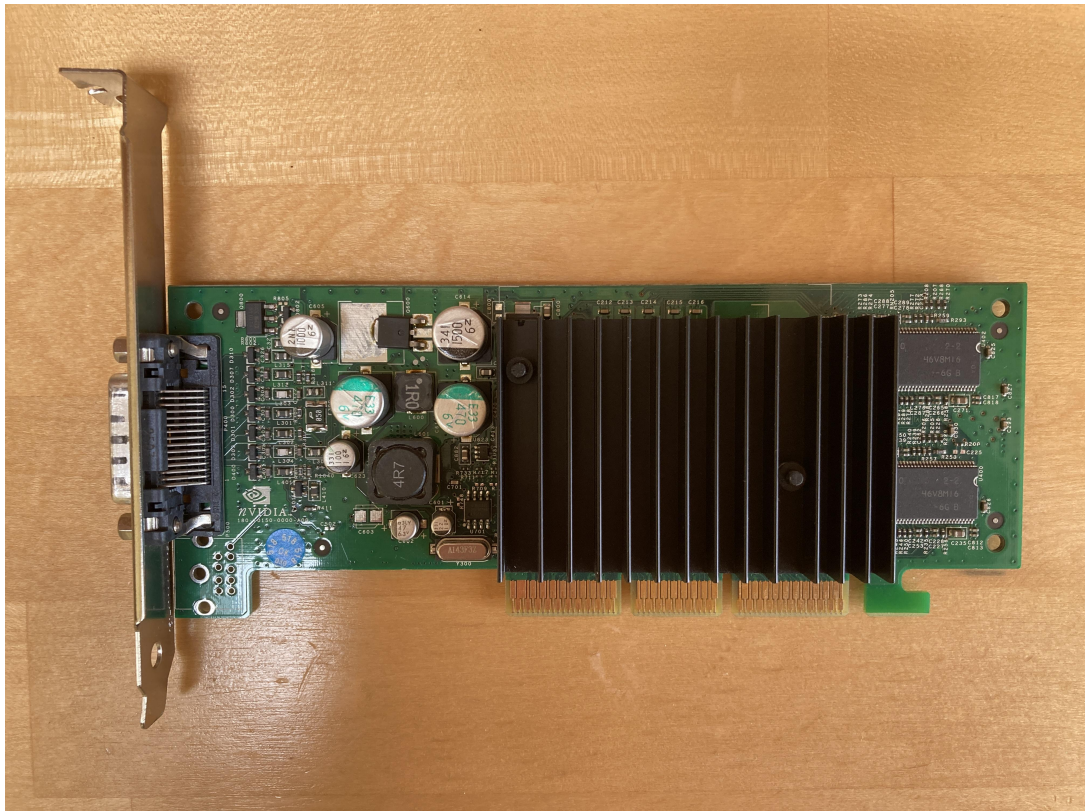
Figure 3: nVidia P150 GPU Card, top view TCD-SCSS-T.20121208.134.02
