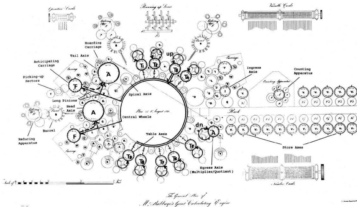
Figure 12. Actions during the main loop of multiplication. A partial product, selected by a digit of the multiplier, is given off by a table axis (in this case T_3 ) and added to the product on the head and tail axes A and A . Simultaneously, the multiplier is stepped down on A to select the next partial product, and the table axes are all stepped up to maintain the correct alignment with the product.
