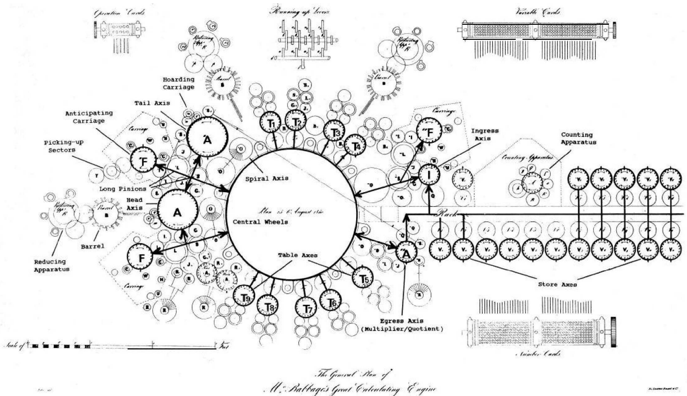
Figure 11. Major registers and data paths of the Analytical Engine. The store axes are arranged along the racks to the right, and communicate with the mill via the “ingress” and “egress” axes, which act as buffer registers. The mill is arranged around the “central wheels,” which act as an internal data bus servicing accumulators A and A and table axes T 1 to T 9 used in multiplication and division. F, F, and F are the figure axes of the three sets of anticipating carry apparatus.
