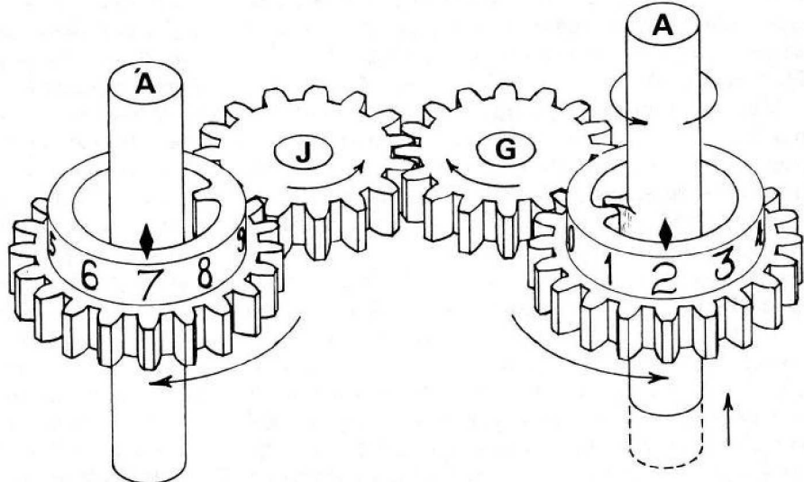
Figure 2. Basic process of addition. A digit is given off by the figure wheel on the right and received by the figure wheel on the left. If the receiving figure wheel is not originally at 0, it will finally come to stand at the sum of its original value and the digit received. This process occurs simultaneously for all digits of numbers.
