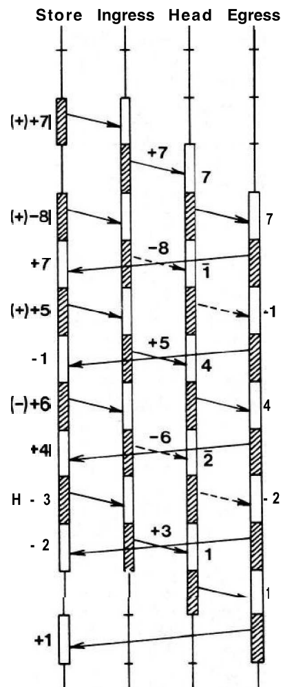
Figure 15. Overlapping of functions in the pipeline for signed addition. The same five operands are accumulated as in Figure 14, but each of the five partial sums is returned to store.
