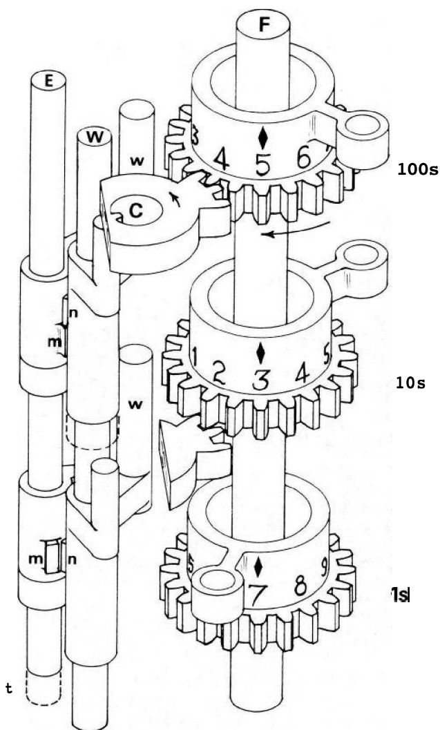
Figure 6. Carry mechanism. The carry warning is raised with its axis E and lifts the carry sector in the cage above into gear with its figure wheel. In the figure there is a carry from the tens into the hundreds cage, but none from the units to the tens.
