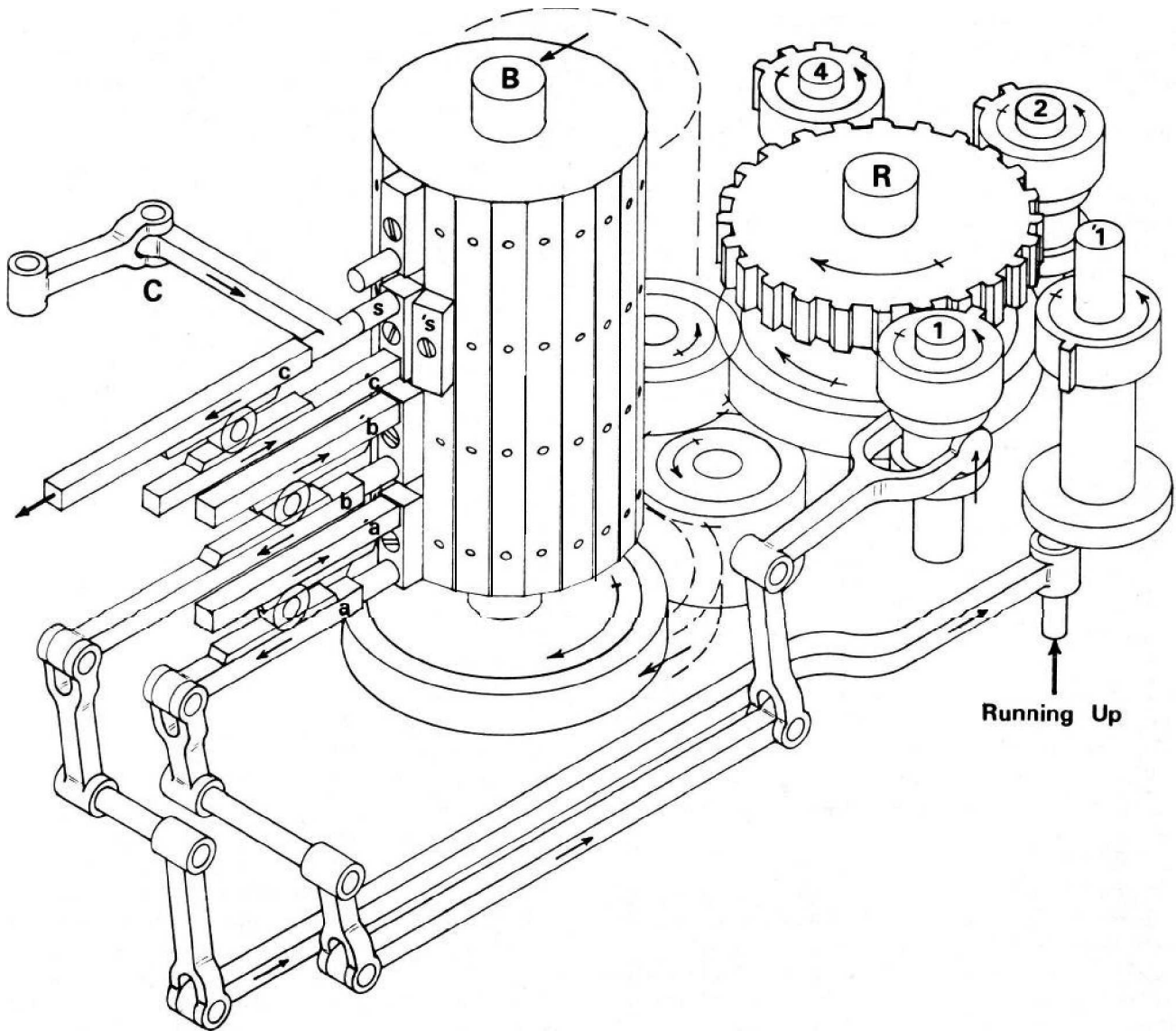
Figure 8. "Barrel" and its "reducing apparatus." 1 A microprogram word is represented by a vertical row of studs screwed to the barrel. These act on the ends of the control levers when the barrel moves sideways. The "reducing sectors" of one, two, and four teeth advance the barrel over the corresponding number of verticals, and several may act in combination at one time. In the figure, reducing sector 1 is put into gear directly by order of the barrel via control lever a. Reducing sector '1' is put into gear by a "running up" from the carry apparatus if enabled to do so by the barrel and lever b. The effect is a conditional transfer. A "conditional arm" is sensed by control lever c to provide an action conditional on a previous event.
