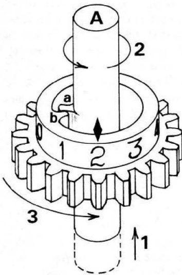
Figure 1. Figure wheel typical of the store and the mill figure axes. The wheel may stand in one of 10 positions to store the digit shown by the index mark. The number may be read by raising the axis until its finger is level with that on the inside of the figure wheel and rotating it through nine digit positions. The figure wheel will come to stand at the 0 position, and a movement proportional to the digit originally stored will be given to the remainder of the mechanism by the gear teeth. The process is termed "Giving Off."
