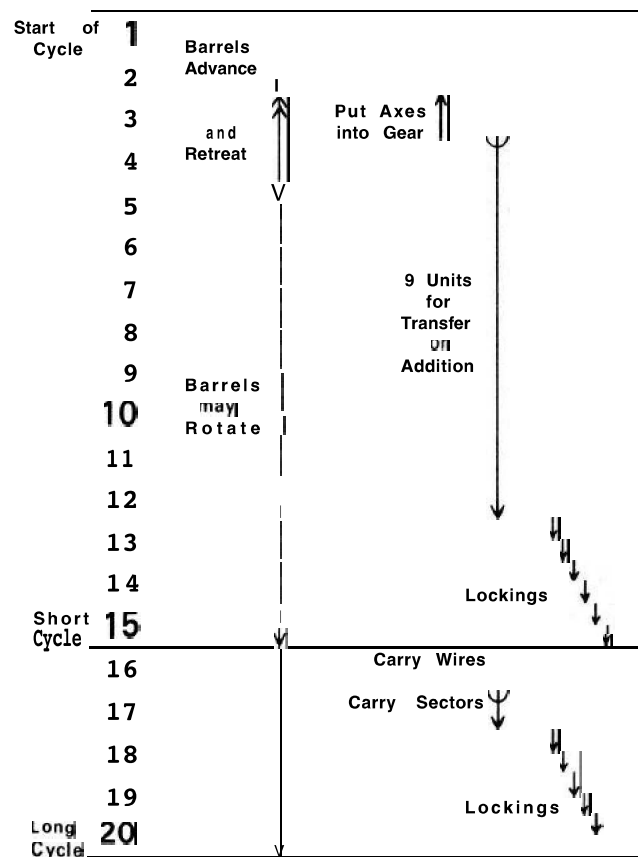
Figure 9. Timing diagram illustrating the events in the basic timing cycle. This figure is similar in style to Babbage's notation of timing.
