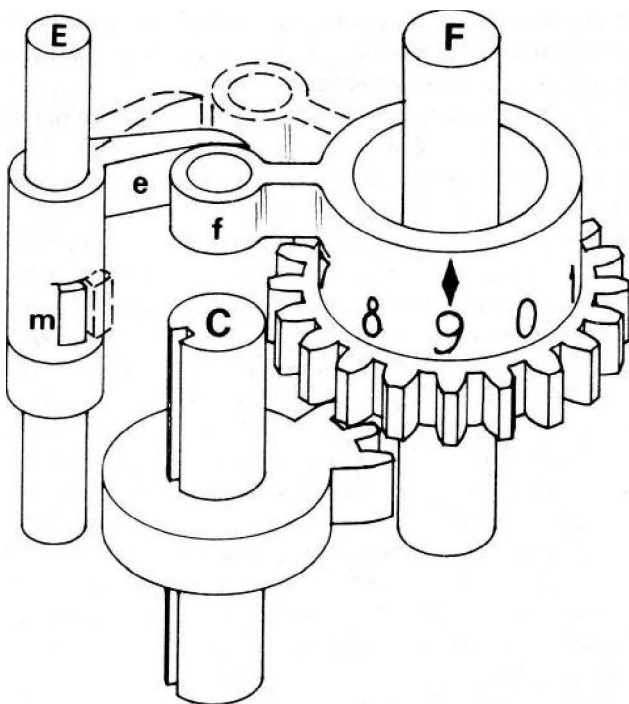
Figure 5. Elements of the carry mechanism. When the carry figure wheel moves past 9 to 0 arm f acts on arm e to rotate the “carry warning” indicating that a carry is necessary into the cage above. A carry from the cage below will raise the “carry sector” on axis C into gear with the figure wheel and advance it by one digit position.
