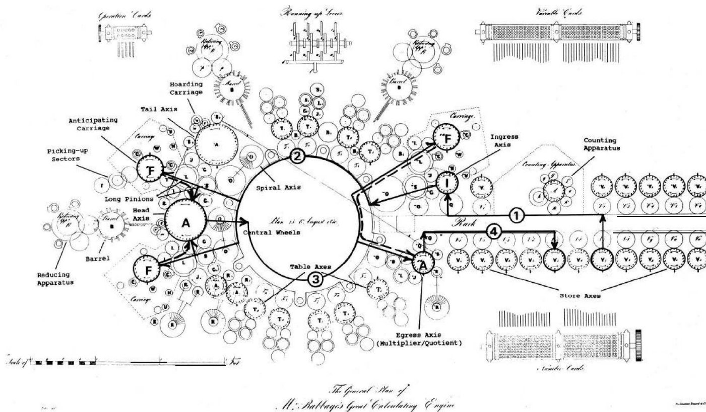
Figure 13. Stages in the pipeline of signed addition. An operand is fetched from the store to the ingress axis \downarrow added to or subtracted from the total on A, the result converted into sign-and-magnitude representation on egress axis "A", and returned to store, in four separate steps that may be overlapped with one another for different operands.
