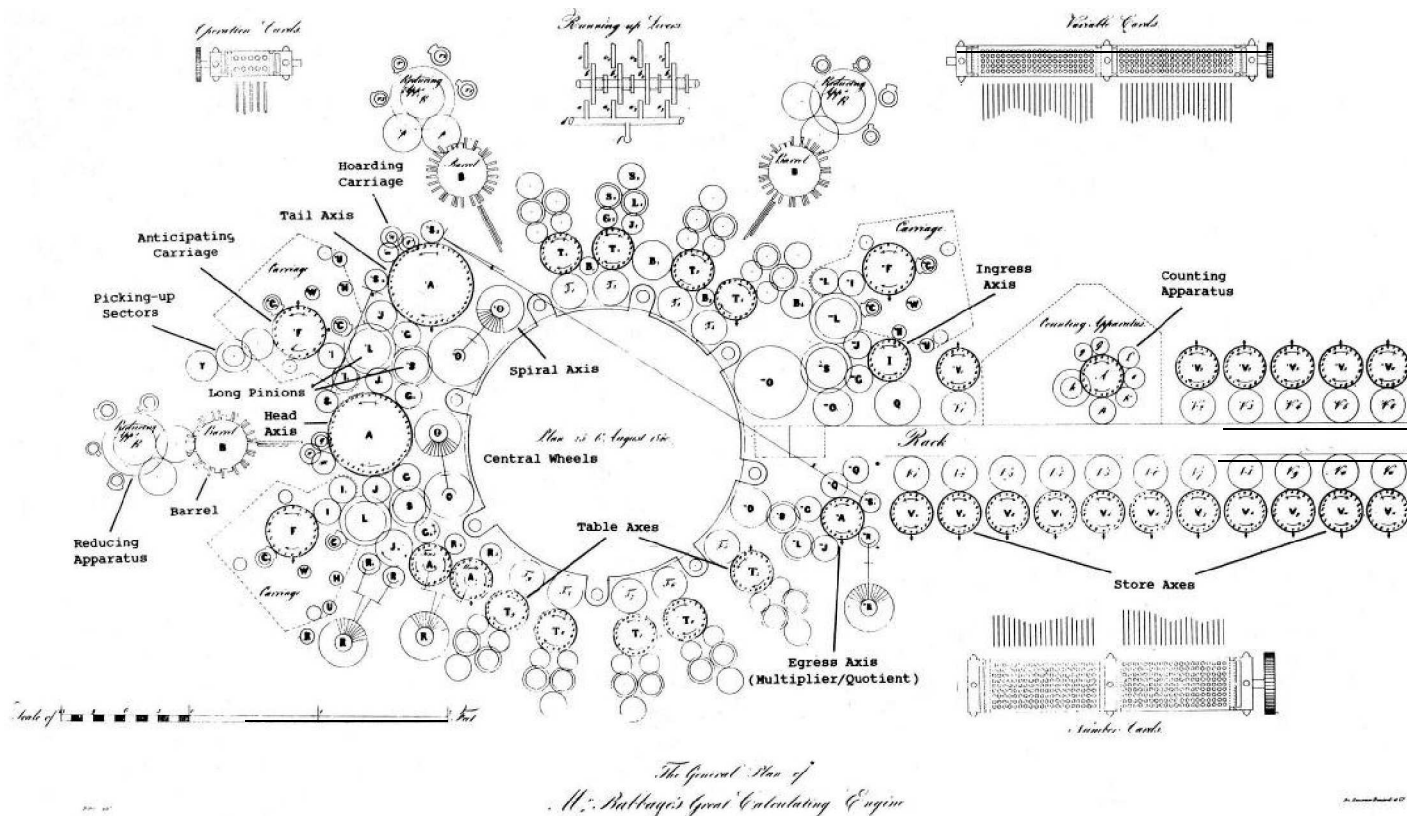
Figure 10. Plan of the general arrangement of the Analytical Engine. It also serves as a functional block diagram, as explained in the text and Figure 11.
