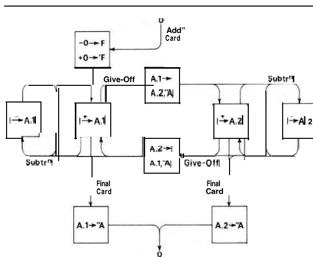
Figure 16. A state transition diagram for one of the barrels in signed addition. The transitions are between the verticals of the barrel controlling the accumulator A and the anticipating carries F and \bar{F} in signed addition (see Figure 13). The transitions between the states, shown by the arrows, are generally multiway conditional branches.
