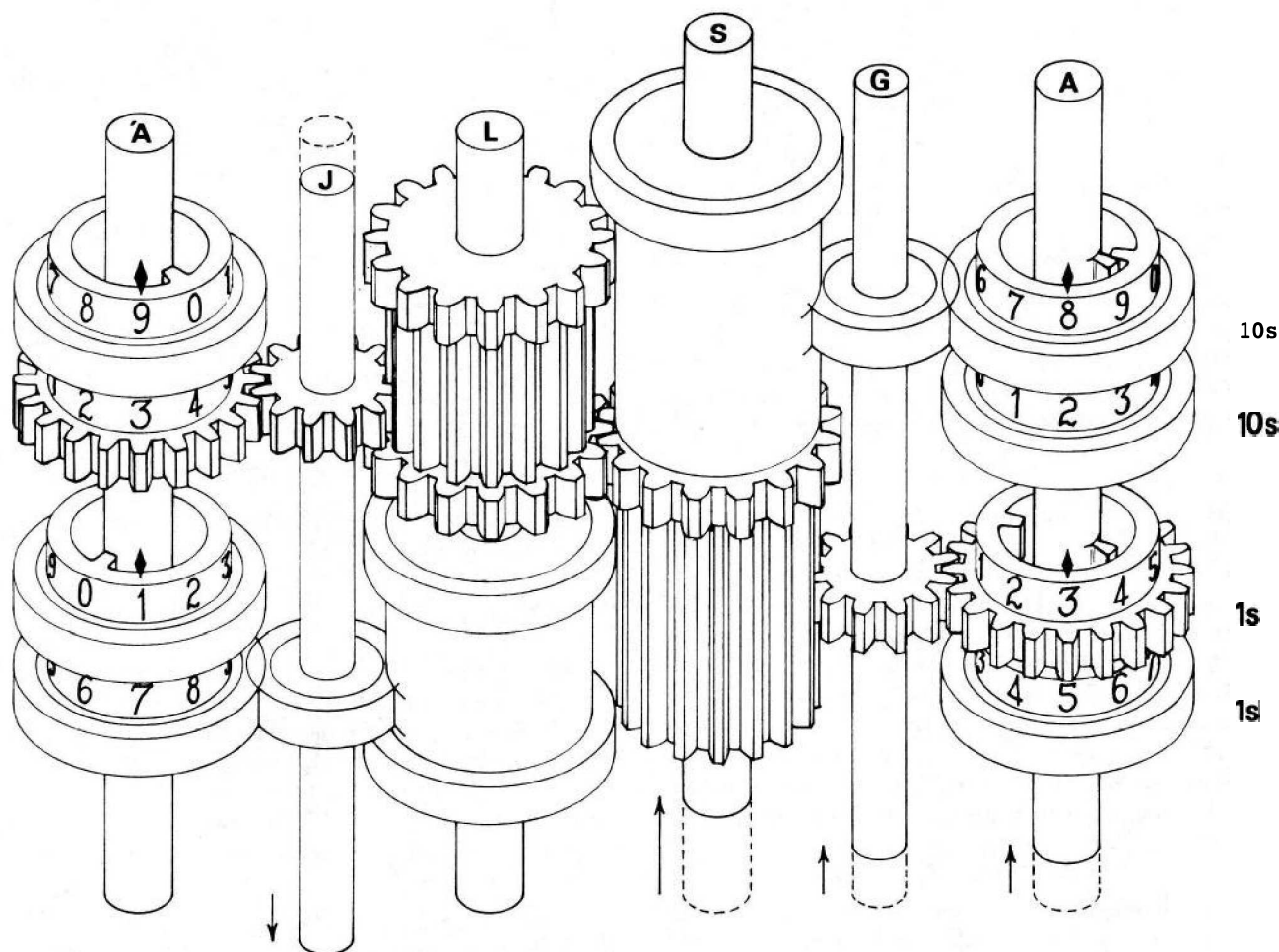
Figure 4. Process of stepping, or multiplication, and division by 10. The "long pinions" S are raised with their axis to engage the long pinions L in the cage above. A number given off will therefore be stepped up a cage, or multiplied by 10. A transfer in the reverse direction will divide by 10.
