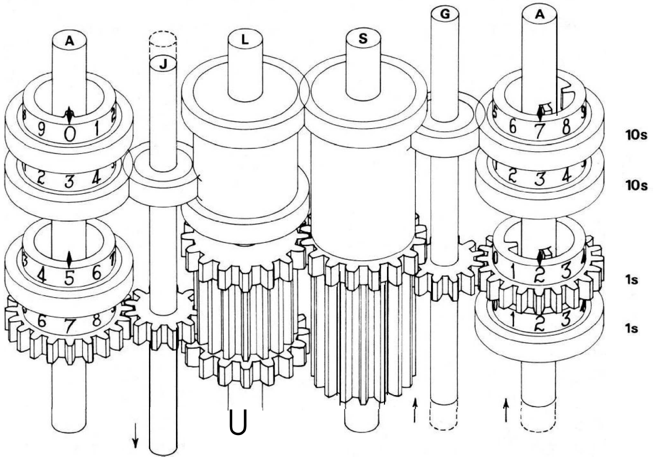
Figure 3. Practical realization of the method of digitwise parallel addition. Two figure wheels are shown in each cage, so two numbers may be stored on each figure axis. In practice the mechanism is arranged in a circle so that the axes A and 'A coincide. A number given off may therefore be received on the alternate set of figure wheels of the same axis.
