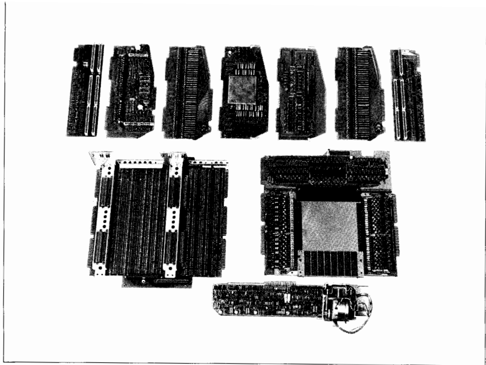
Fig. 4. Printed circuit boards which make up the arithmetic unit are, left to right at top, side board, control logic, flip-flop, core and drivers, core sense amplifiers and inhibit, flip-flop, and side board. Large board at the lower left is the multilayer instruction board and the program ROM is at the right. The magnetic card reader and its associated circuitry is at the bottom.
