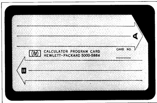
Fig. 9. Magnetic programming card can record two 196-step programs. To prevent accidental recording of a new program over one to be saved, the corner of the card is cut as shown.
