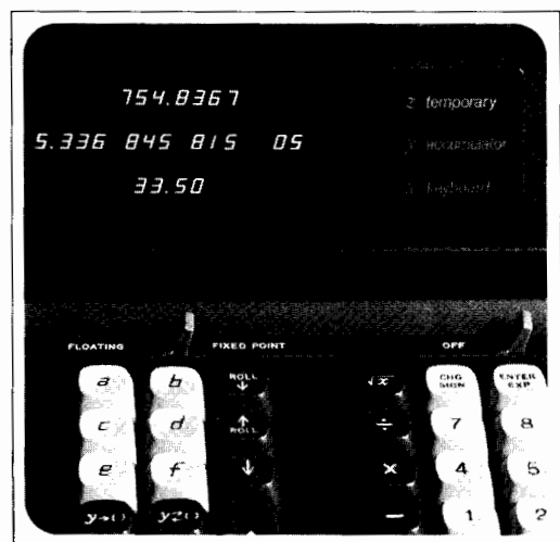
Fig. 1. (left) This new HP Model 9100A Calculator is self-contained and is capable of performing functions previously possible only with larger computers. Fig. 2. (right) Display in fixed point with the decimal wheel set at 5. The Y register has reverted to floating point because the number is too large to be properly displayed unless the digits called for by the DECIMAL DIGITS setting is reduced.
