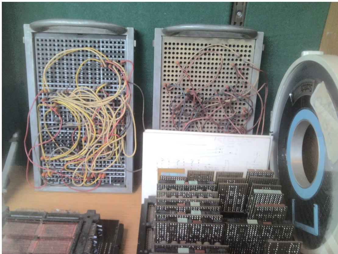
Figure 1: 2 x IBM 870 Patch Panels front view
